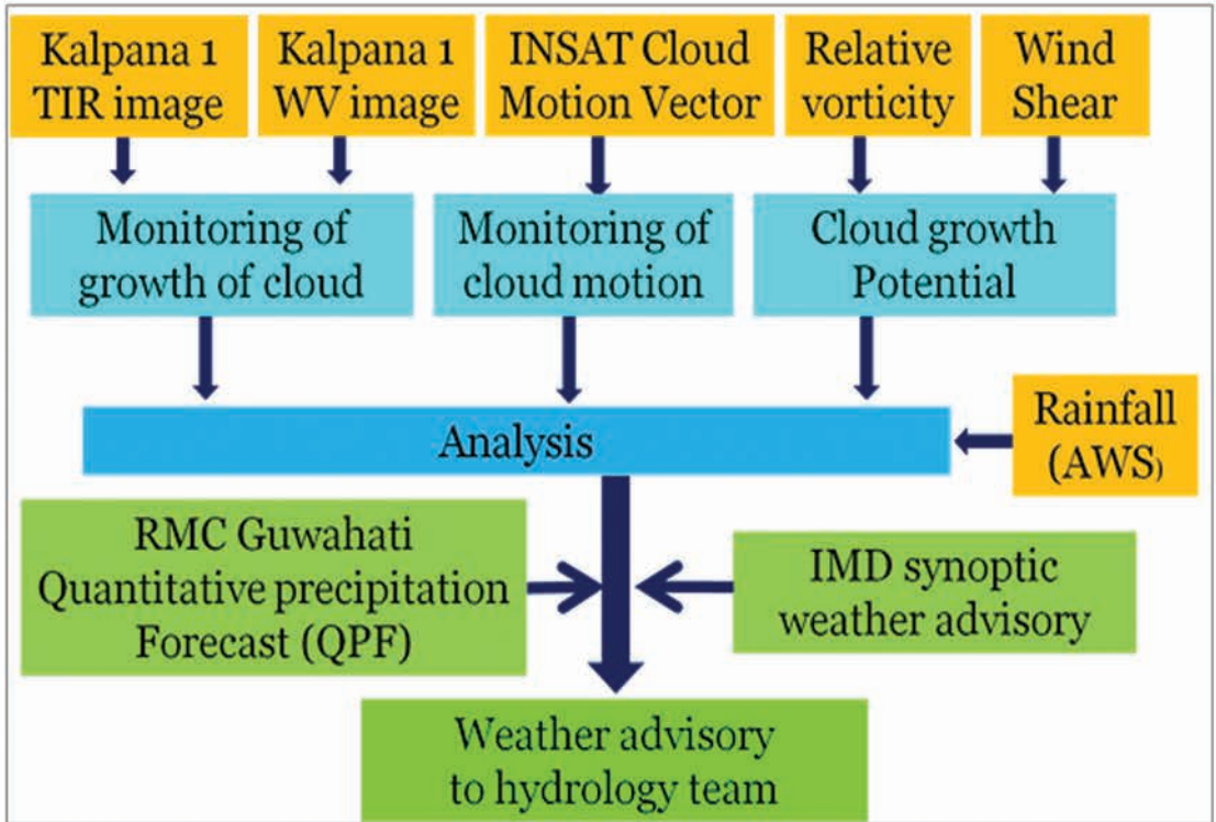
Fig.8: Methodology flow chart for synoptic and meso scale rainfall forecast
