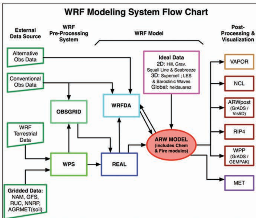
Fig.6: WRF Modelling system flow chart
