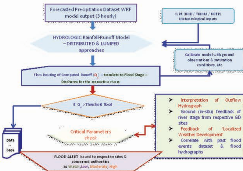
Fig.11: The HEC-HMS operational block
